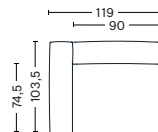
Left armrest Art. S1962 W90/119 x D74,5/103,5 x H37/67 cm Armrest D29 cm
